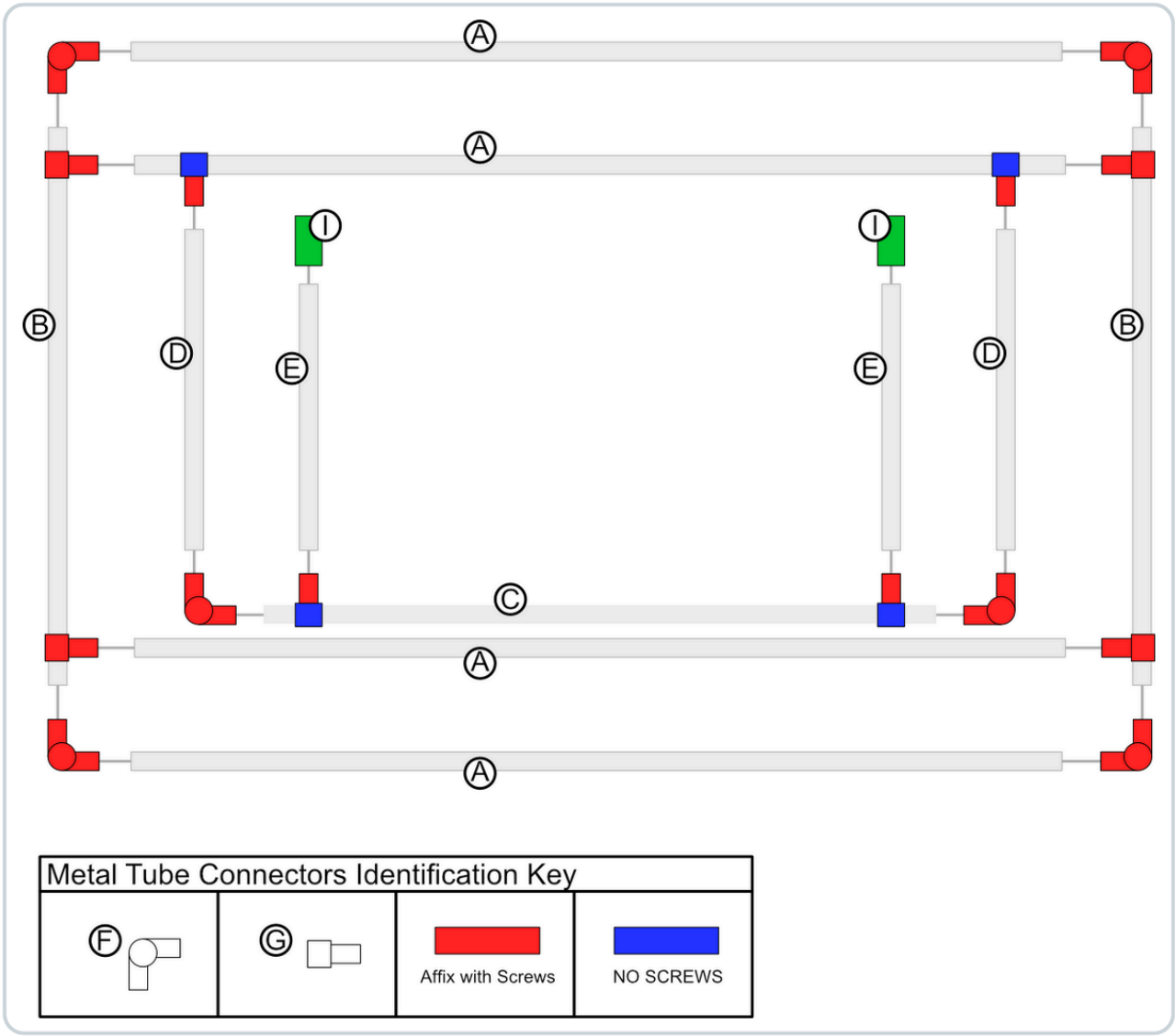
Figure 7: Exploded folded-state component and connector-fastening map.
