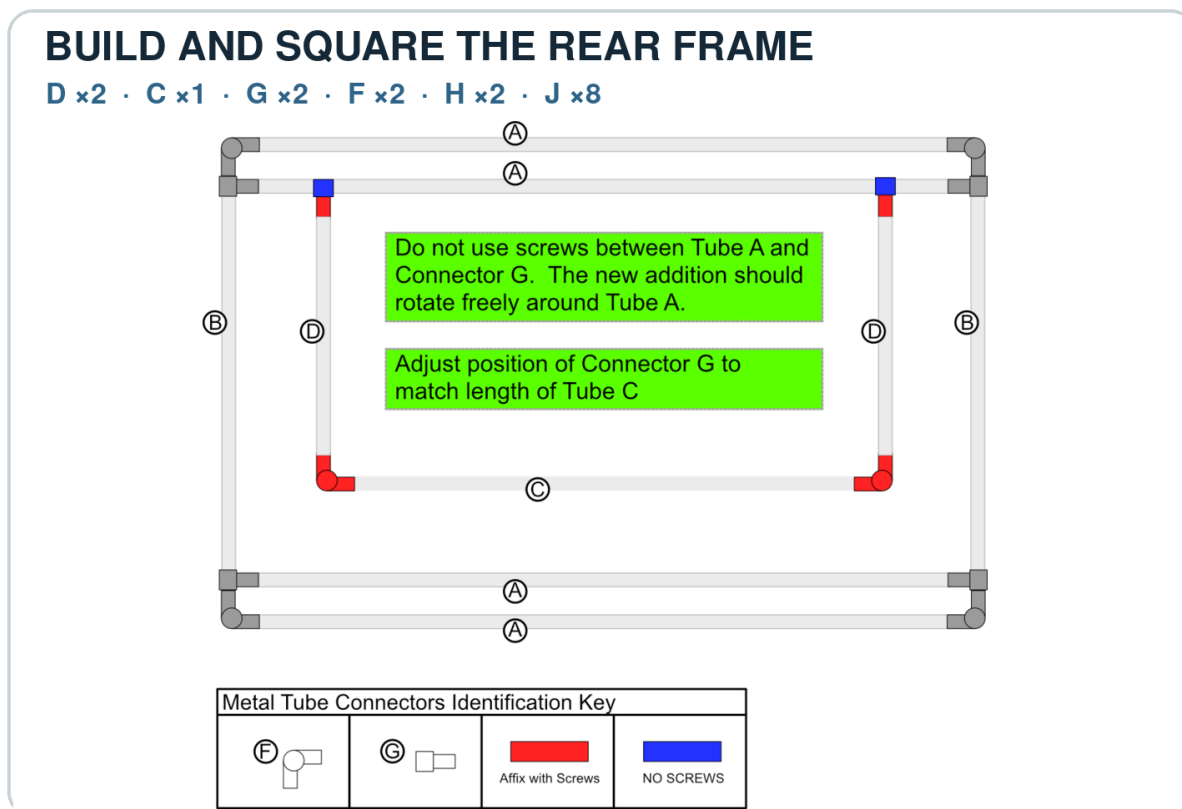
Figure 10: Stage 3 rear-support-frame assembly and hinge fastening.
