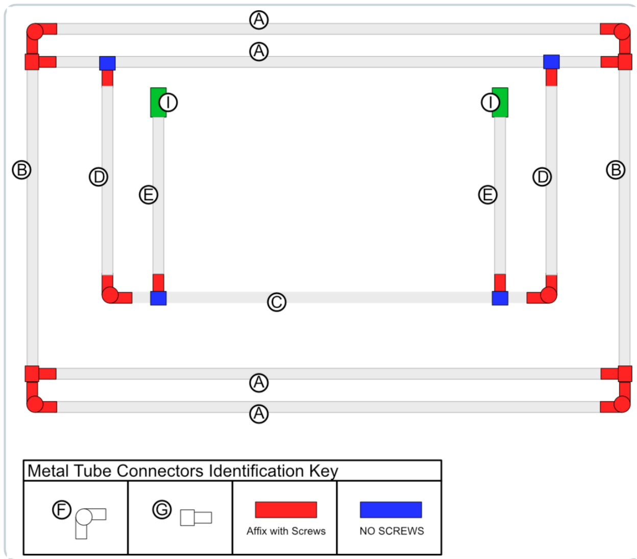
Figure 6: Folded-state component and connector-fastening map for the finished frame.
